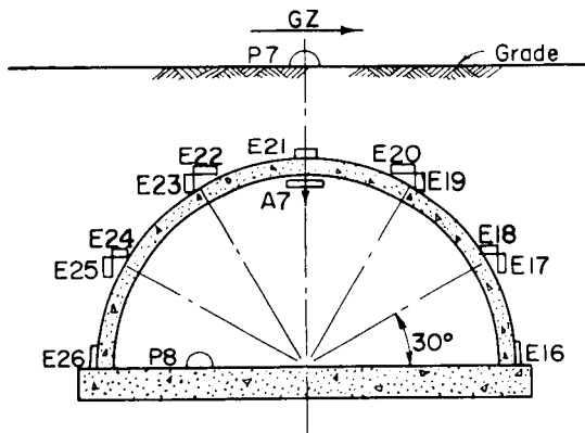
SECTION E-E
